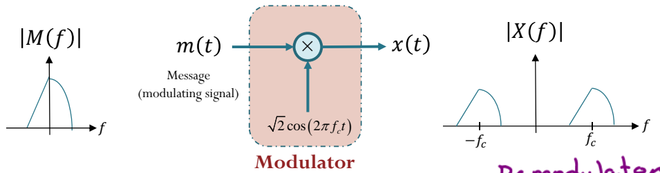
Figure 25: DSB-SC modulation.
