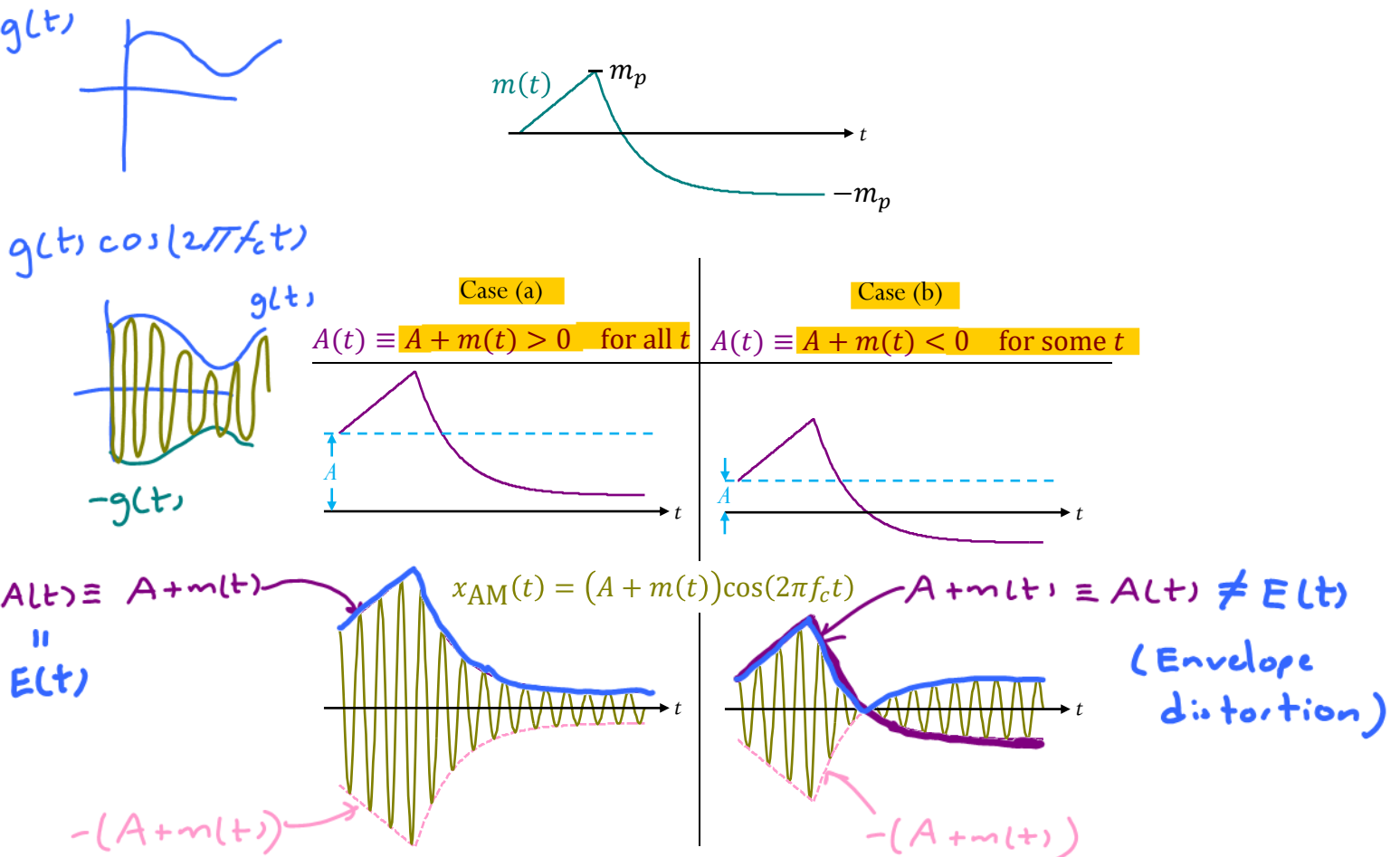
Figure 26: AM signal and its envelope [6, Fig 4.8]
