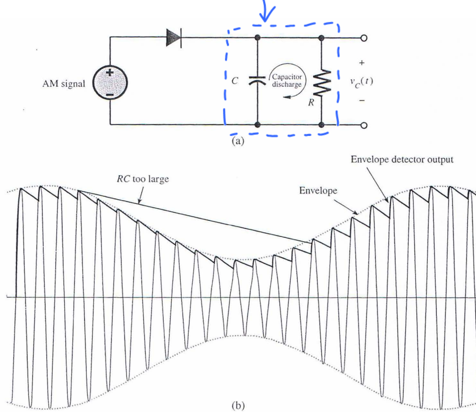
Figure 29: Envelope detector for AM [6, Fig. 4.11].
