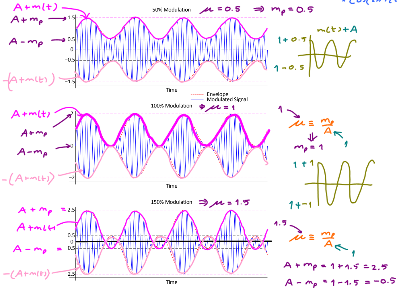
Figure 27: Modulated signal in standard AM with sinusoidal message
