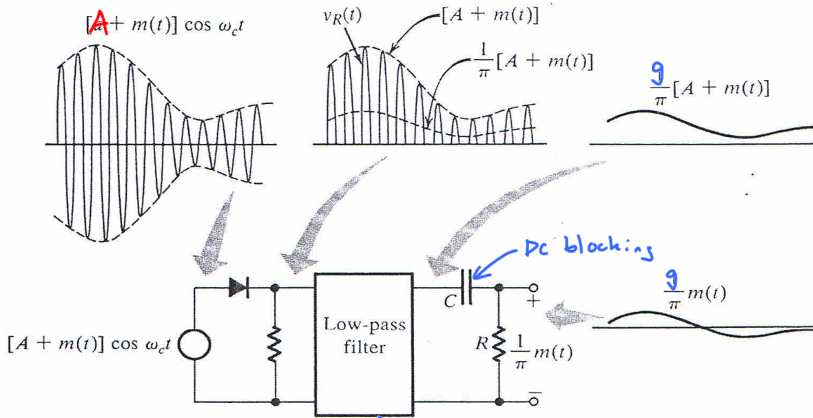
Figure 28: Rectifier detector for AM [6, Fig. 4.10].
